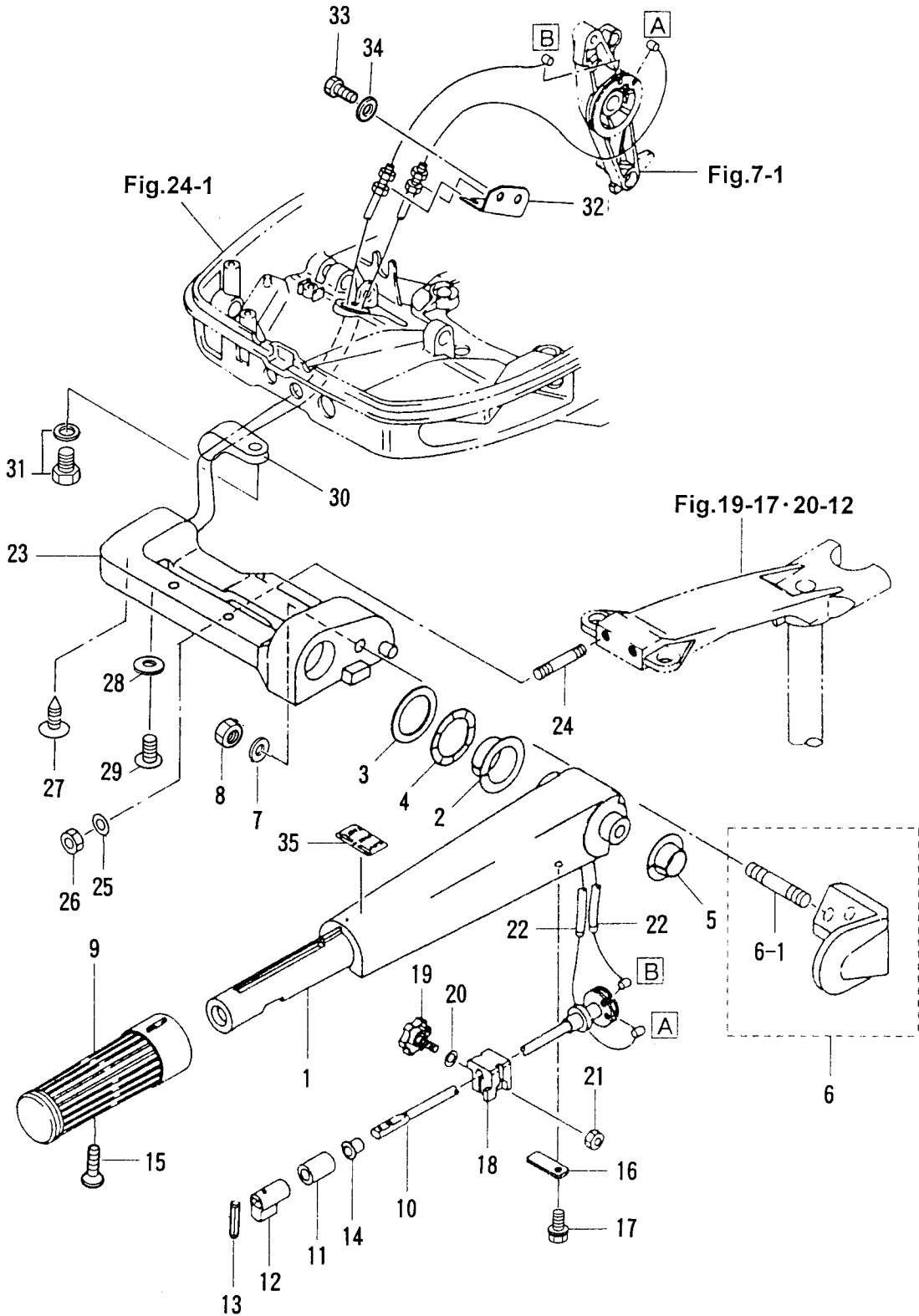
Fig. 8 STEERRING HANDLE (F Type)
