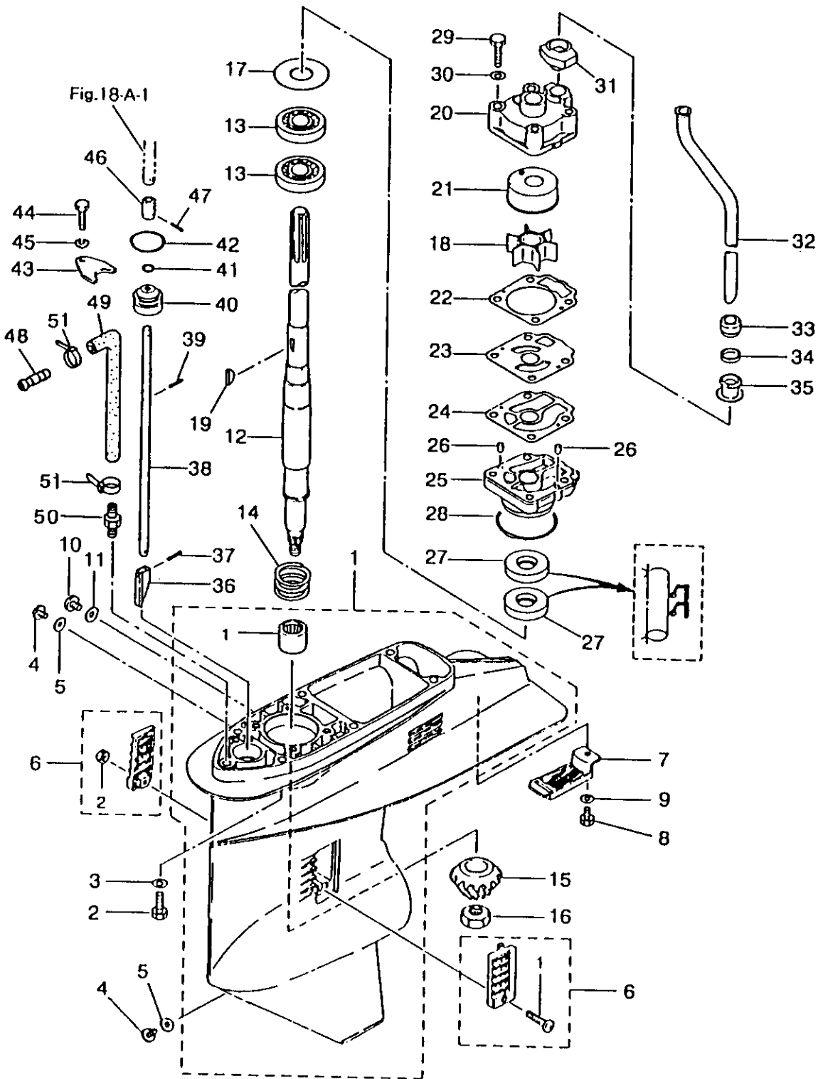
FIG. 16-A GEAR CASE(DRIVE SHAFT)
