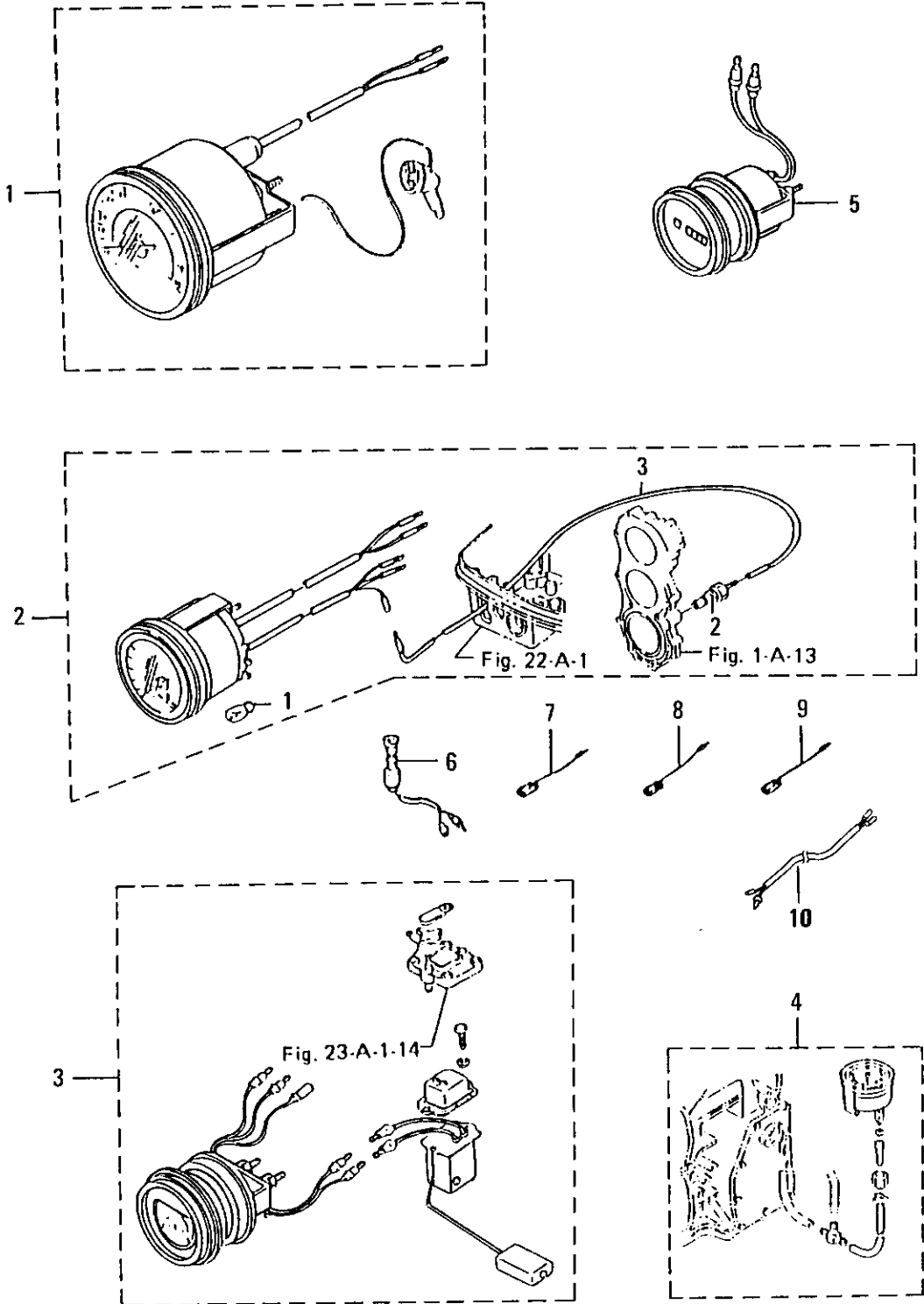
FIG. 26-A OPTIONAL PARTS (1) ACCESSORIES (METER)
